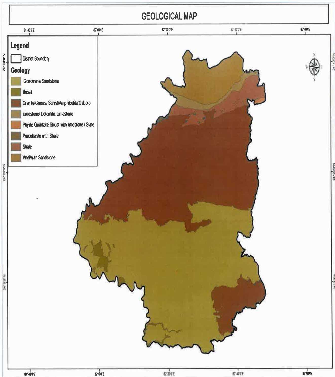
Figure 4 Geological Map of the District
