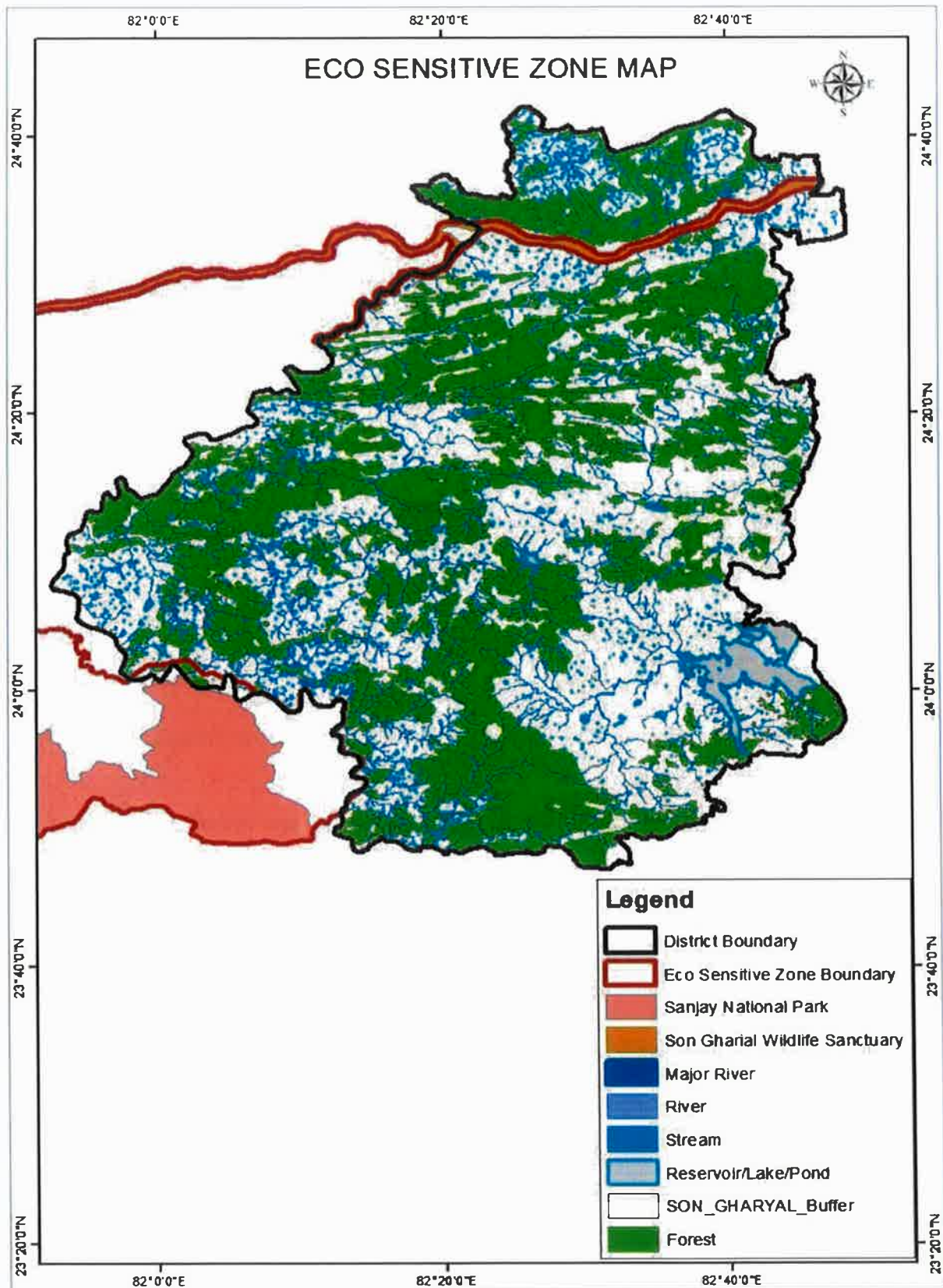
Figure 13 Eco-sensitive map of the District
