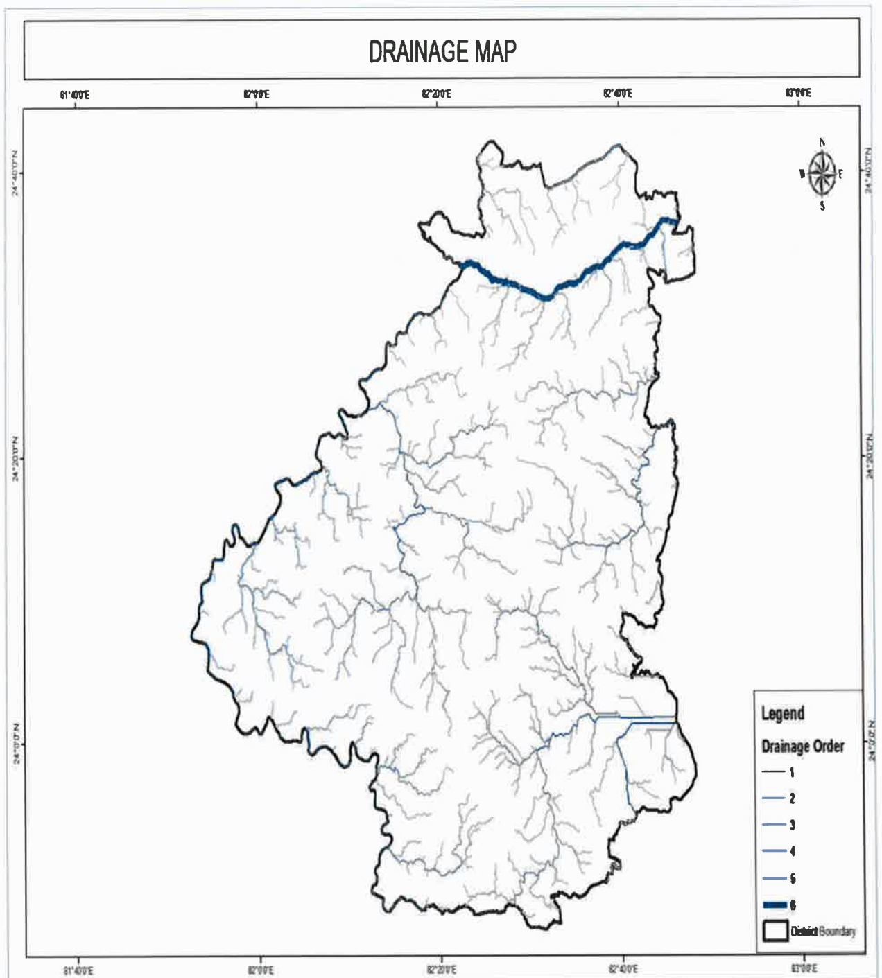
Figure 6 Drainage Map of the District
