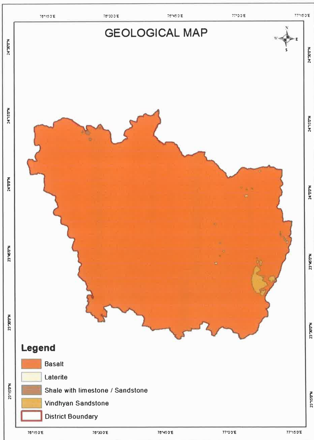
Figure 4 Geological Map of the District
